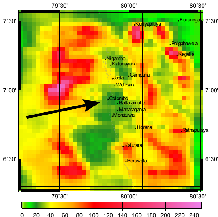
Figure 6: Accumulated rainfall (mm) from 2-3 May 2007 rainfall event simulation. The prevailing surface wind direction is marked by the arrow.
