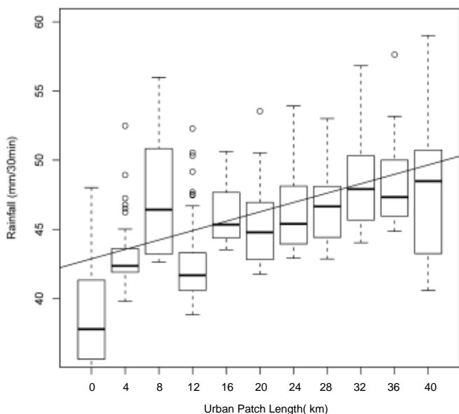
Figure 2: The largest 25% of grid-level rainfall observed over the 60km monitoring area. All 30 min rainfall values of each ensemble set (i.e. all simulations for a specific length of urban patch) were pooled and sorted in the order of descending intensities. Then the first 25% were used to produce the corresponding box plot.
