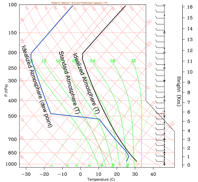
Figure 1: The model domain for idealized experiments (Top). Log-P-Skew-t plot for the atmosphere profile (Bottom).
