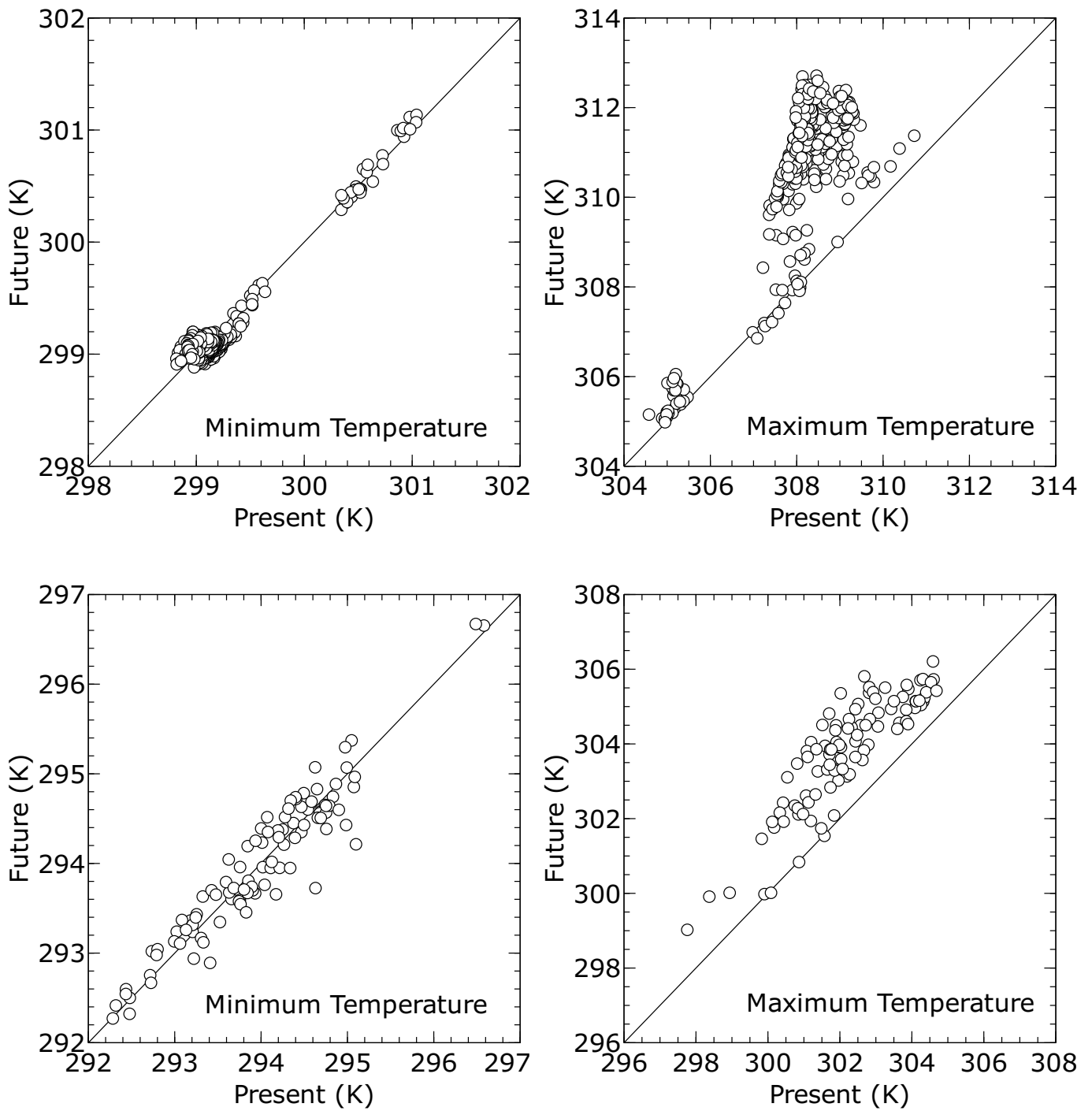
Figure 8: Simulated maximum (daytime) and minimum (night-time) Temperature in Dhaka (top) and Taipei(bottom) during the event.
