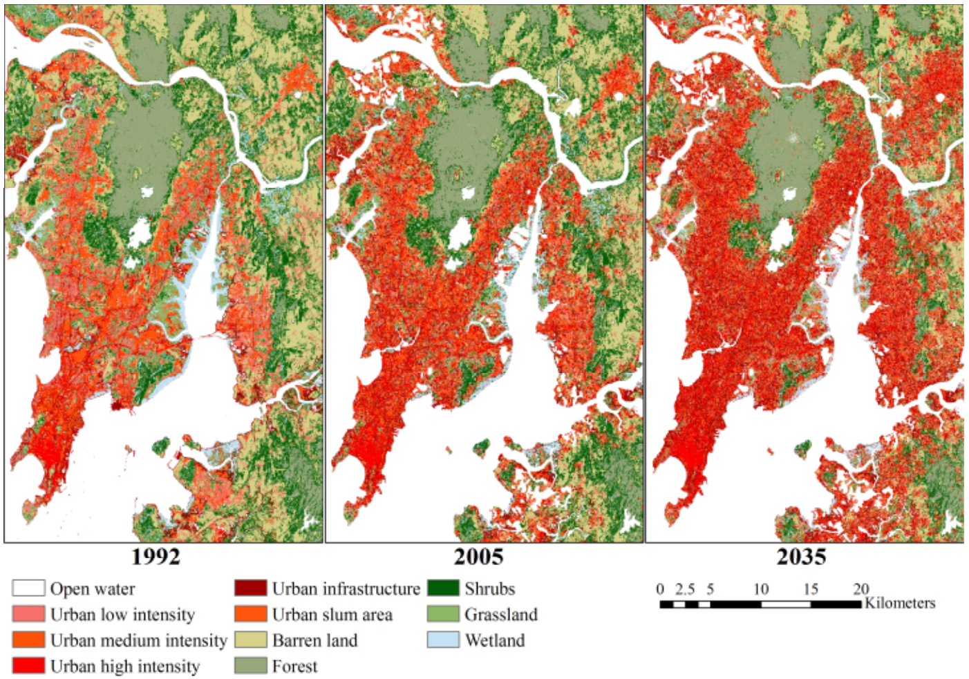
Figure 9: Land-use classifications derived from LandsAT data (1992, 2005) and Dynamica EGO simulation (2035).
