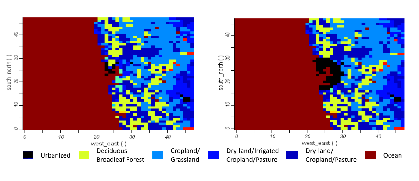
Figure 4: The landuse transformation introduced in the semi-idealized study for the case of Colombo, Sri Lanka. Left: Current, Right: Transformed
