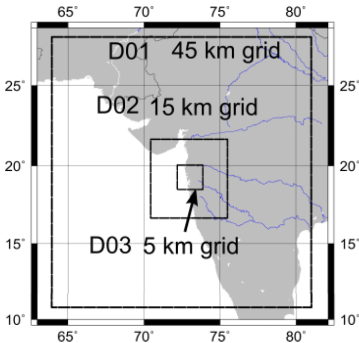
Figure 5: Nesting scheme used for Semi-Idealized studies. The case of Mumbai City is shown.
