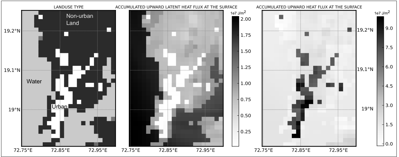
Figure 13: Accumulated latent heat flux (center) and accumulated total heat flux (right) for 2005 July Mumbai case (Event 4), 'present scenario'. Corresponding landuse map (simplified) is shown on the left. Urban areas decrease the latent heat flux dramatically, while increasing sensible heat flux (hence the total heat flux is increased).
