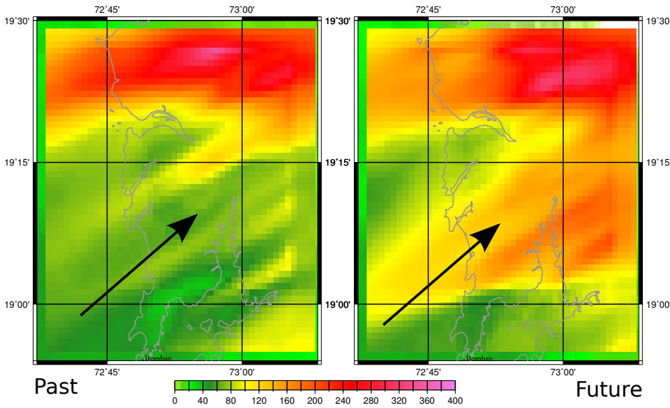
Figure 14: Total rainfall accumulations (mm) during the 2007 July rainfall event simulation. The prevailing surface wind direction is marked by the arrow.
