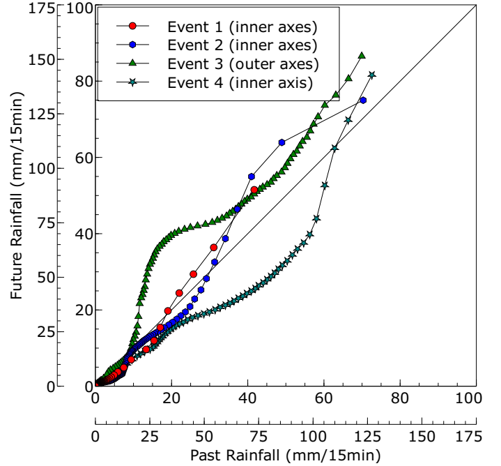
Figure 11: Quantile-quantile plots of the simulations of four events in Mumbai.
