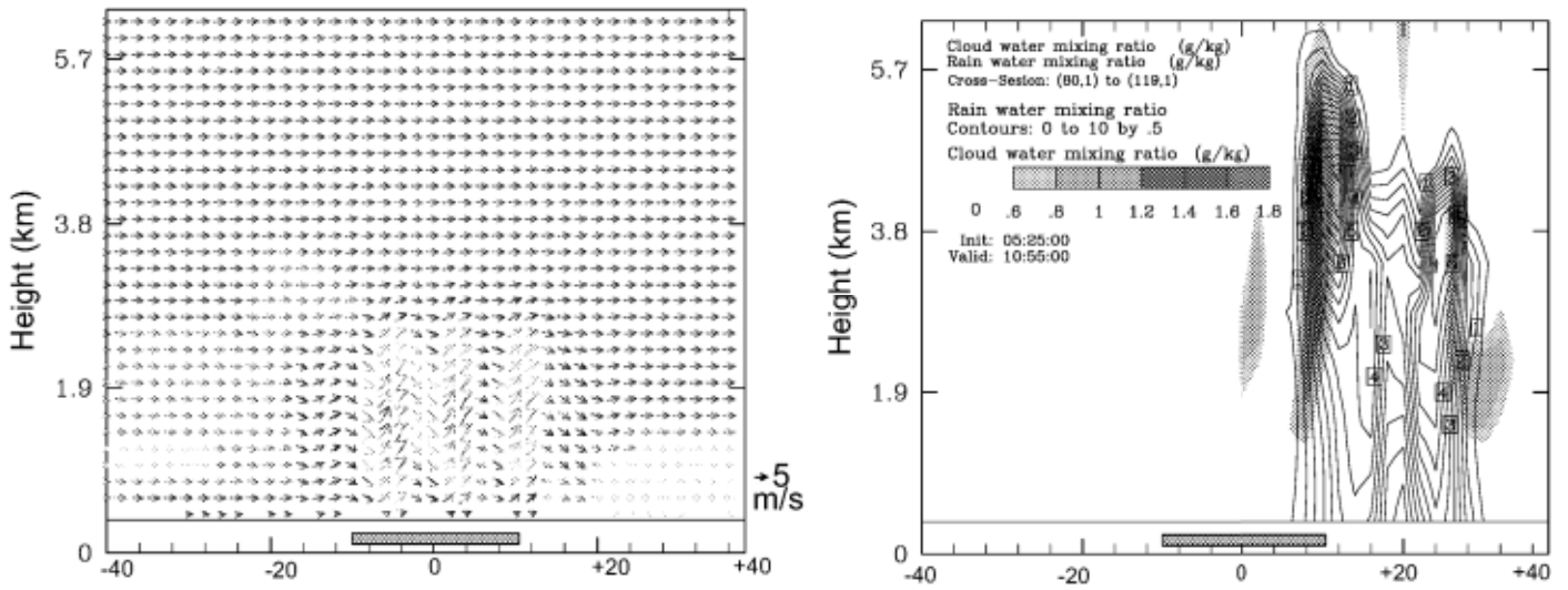
Figure 3: Cross sections of a simulation with 20 km urban patch. Left: Wind vectors at 09:55 hrs (with vertical exaggeration of 50) shows the initiation of convective activity aloft the urban patch (gray bar). Right: Cloud formation and rainfall at 10:55 hrs. The precipitation starts at the lee-side of the urban-patch.
