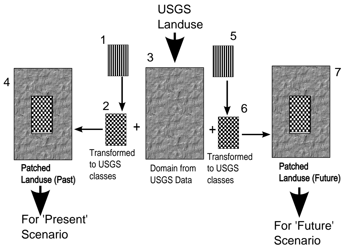
Figure 10: The landuse patching process. (1) 'Present scenario' landuse map produced by urban growth simulation model, based on its own landuse classes. (2) Same map transformed to USGS 24 category classes. (3) The Landuse map created using original USGS landuse data. (4) The patched landuse map used in WRF model simulations for 'Present scenario'. (5),(6),(3) and (7): same procedure for 'Future Scenario'.
